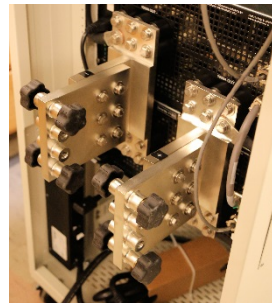
Real 2000 Amp (Front and Rear) total of 44 cm (17.5 inches) is all that is required for the 2 CS 1000 A Sources
