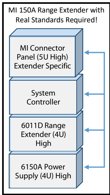
Guildline's 6623A-150 Extender Diagram Below Yes - Only One Standard
