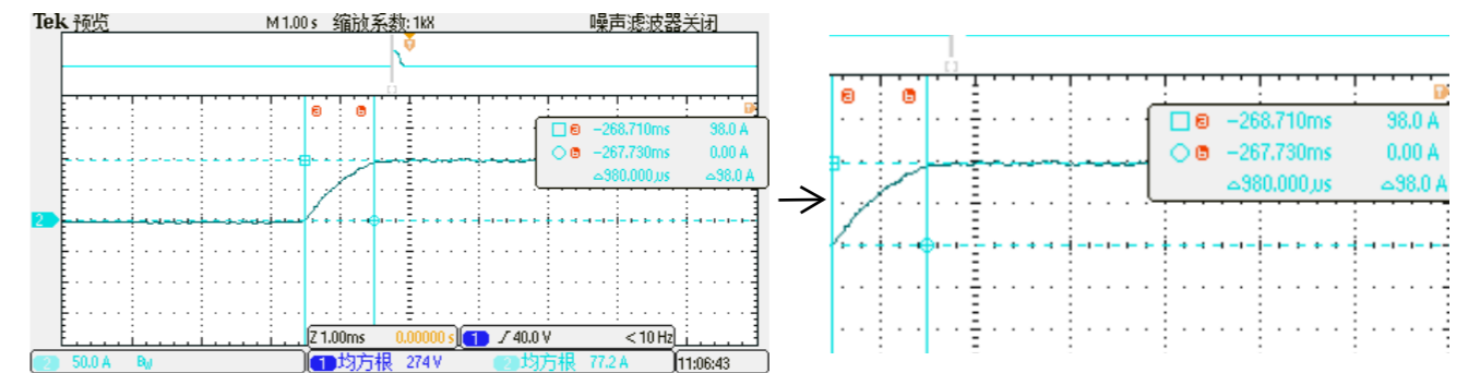
Current Rise Time (0%~90%) T_{Rise} \leq 1ms (Example ESD 50-400-125-R)
